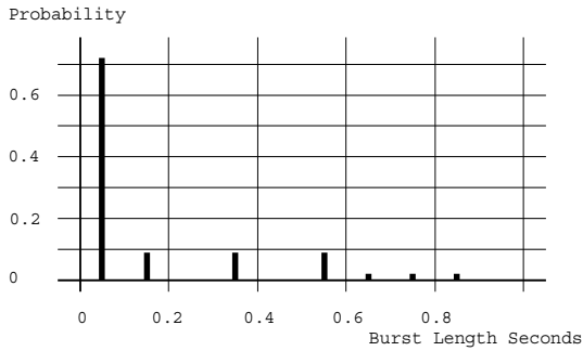
Figure 3: Probability Distribution Of Burst Length
