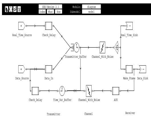
Figure 5: Simulation Model
