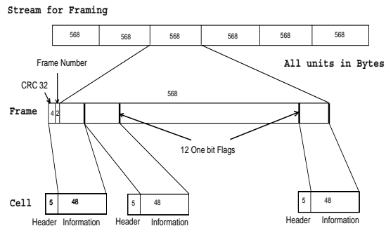
Figure 4: Proposed Convergence Sublayer AAL
