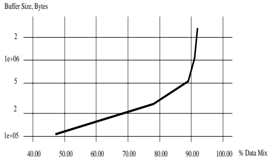
Figure 7: Transmitter Buffer Required For No Framed Cell Loss
