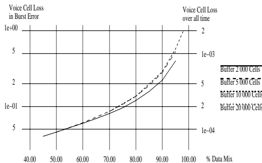
Figure 9: Real Time Cell Loss, Varying Buffer Size
