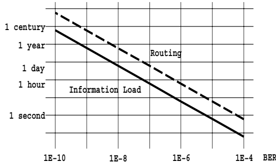
Figure 1: Loss For 155-Mb/s Link For Various Bit Error Rates (BER)
