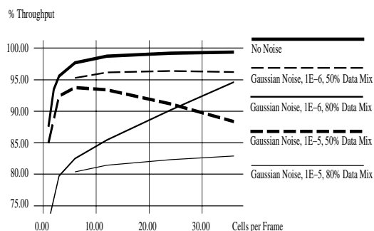
Figure 10: Variation Of The Number Of Cells In A Frame
