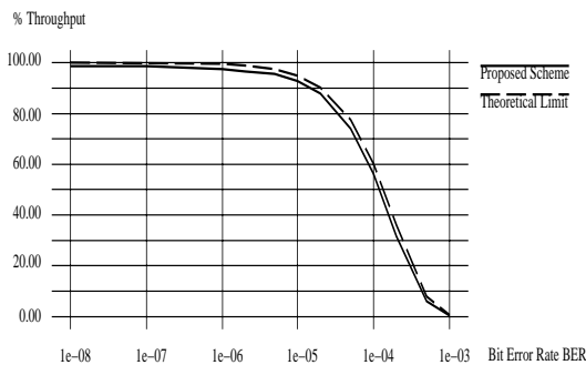
Figure 11: Comparison Of Proposed Scheme With Theoretical Limit
