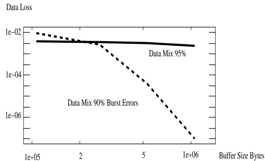
Figure 8: Effect Of Varying The Buffer Size
