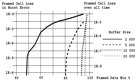
Figure 6: Framed Data Loss For Burst Error, Varying Buffer Size
