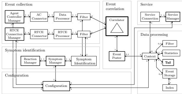
Figure 2: RTCE internal structure
